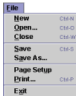
Drop-down menu
