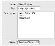
MacOS X
