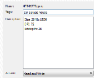
Windows
